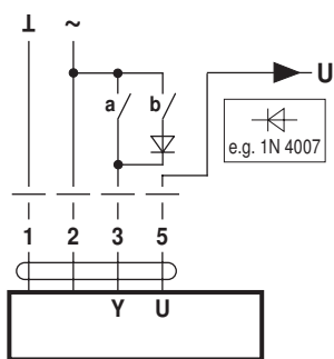
Control 3-point
